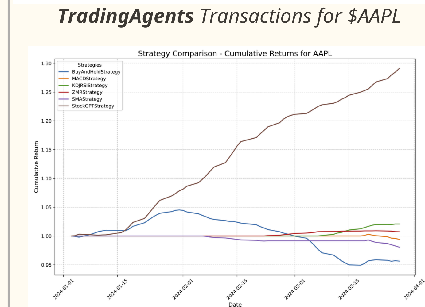
TradingAgents Cumulative Returns
